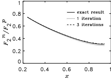
FIG. 8. Neutron to proton structure function ratio extracted from the F_2^{3\text{He}}/F_2^{3\text{H}} ratio via the iteration procedure. The input is F_2^n/F_2^p = 1 , and the ratio after \sim 3 iterations is indistinguishable from the exact result.
