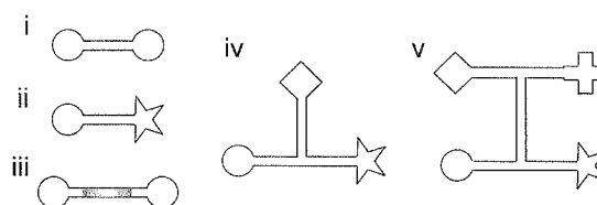
Figure 1: Representative captamers. Aptameric heads are depicted as different shapes. (i) Homodimer, (ii) Heterodimer, (iii) Homodimer with shaded internal transcription factor binding site, (iv) Trimer based upon a 3WJ scaffold, (v) Tetramer based upon two 3WJ scaffolds.
