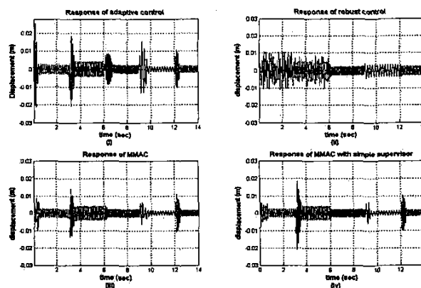
Fig.1 Responses for cases (i)-(iv).
