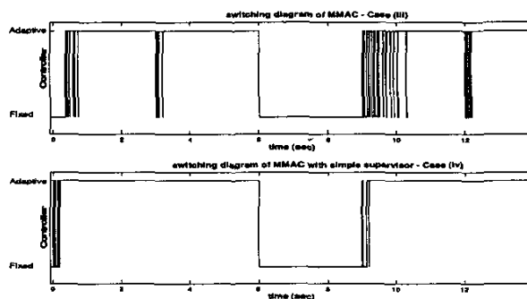
Fig 2. Switching diagrams for cases (iii) and (iv).
